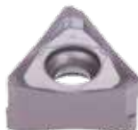
TNGU12-MJ s wiper hranou APMX = 11 mm
